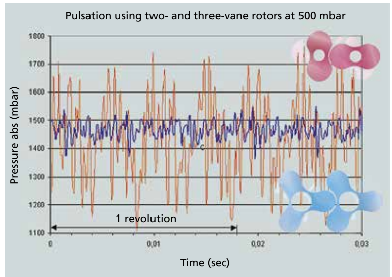
Red: usual lobe vacuum pumps Blue: RPL vacuum pumps
